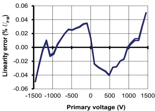
Figure 17: Typical linearity error at 25^\circ\text{C}
