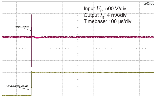
Figure 13: Typical common mode perturbation (1000 V step with 6 \text{ kV}/\mu\text{s} , R_M = 100 \Omega )
